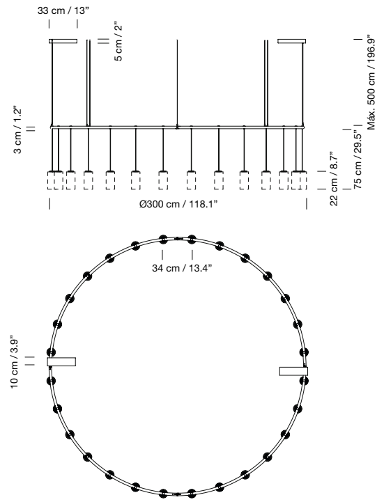
Rectangular canopy
