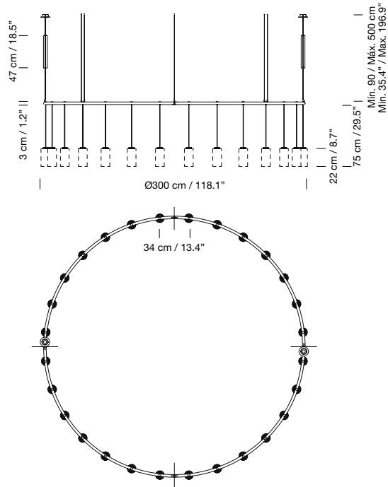
Circular canopy
