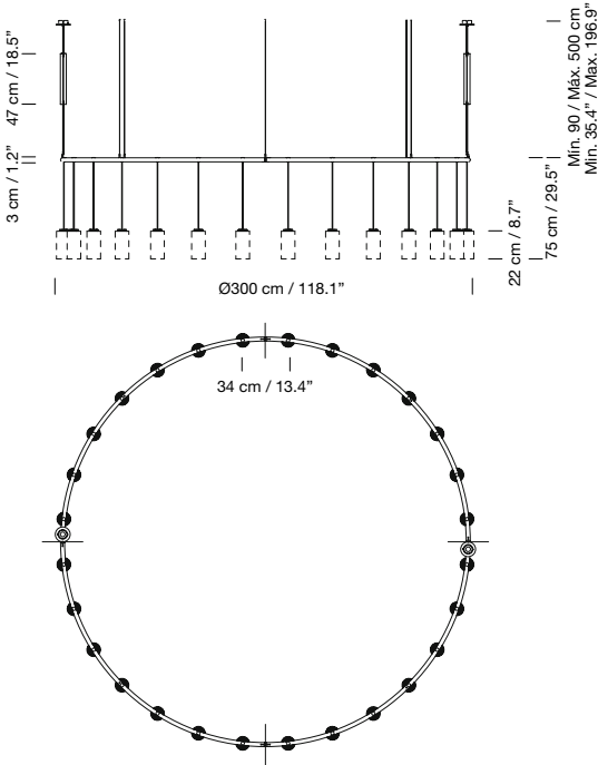
Circular canopy
