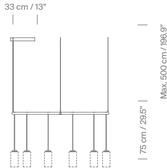
Rectangular canopy / Florón rectangular
