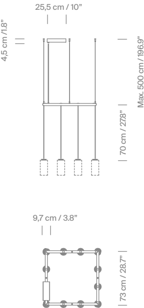
Rectangular canopy / Florón rectangular
